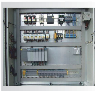
PLC Control Panel
